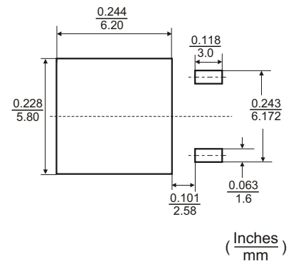
Pad Layout
