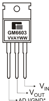
TO-220
