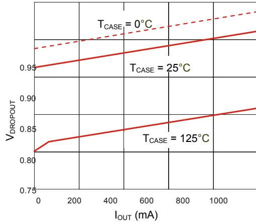
Figure 1. Dropout Voltage vs. Output Current
