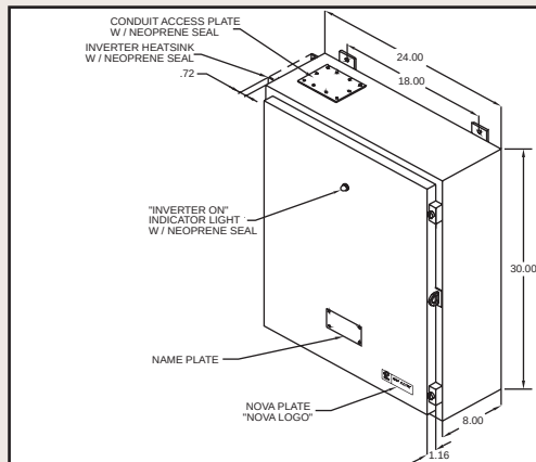
TYPICAL GH2K60-600 CABINET
