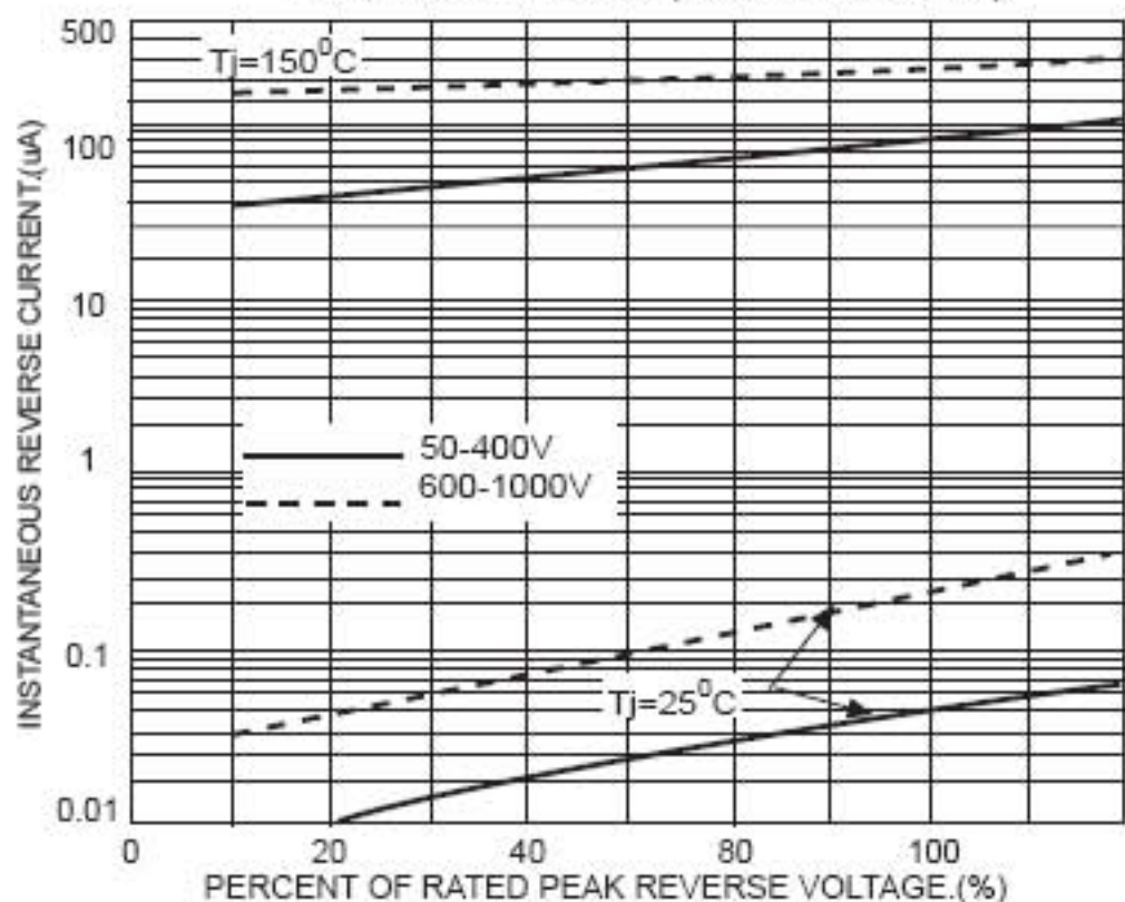
FIG.4-TYPICAL REVERSE CHARACTERISTICS PER BRIDGE ELEMENT(GBU4005 THRU GBU410)
