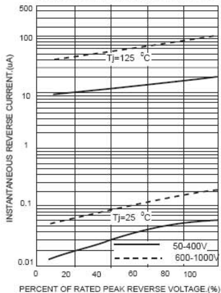
FIG.4-TYPICAL REVERSE CHARACTERISTICS PER BRIDGE ELEMENT(GBU6005 THRU GBU610)
