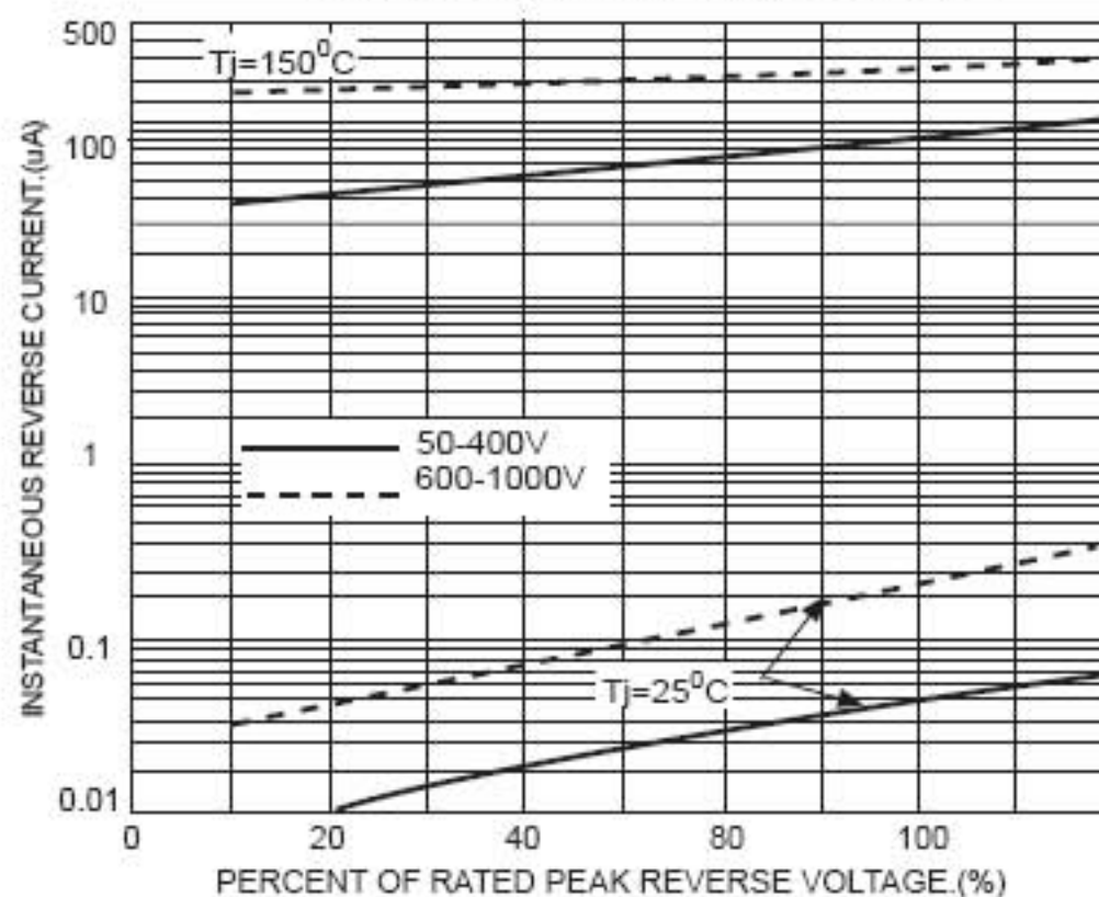
FIG.4-TYPICAL REVERSE CHARACTERISTICS PER BRIDGE ELEMENT(GBU6005 THRU GBU610)
