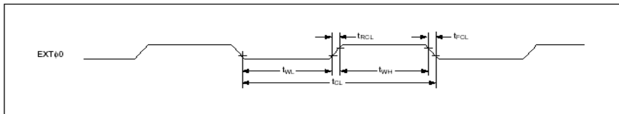
External oscillator signal timing
