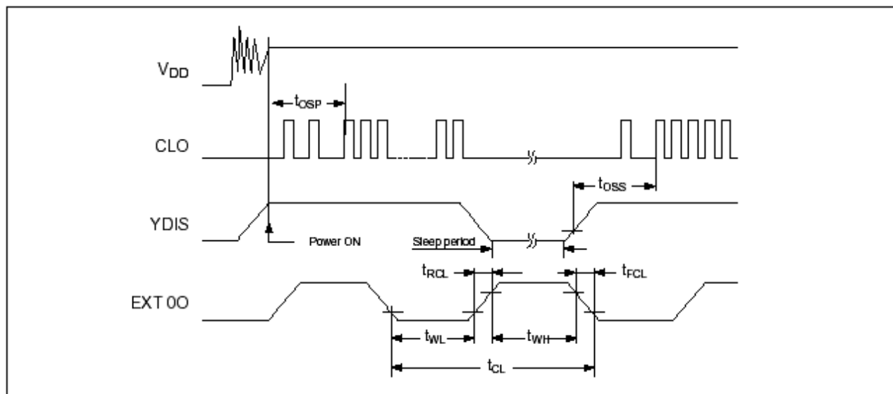
Oscillator timing
