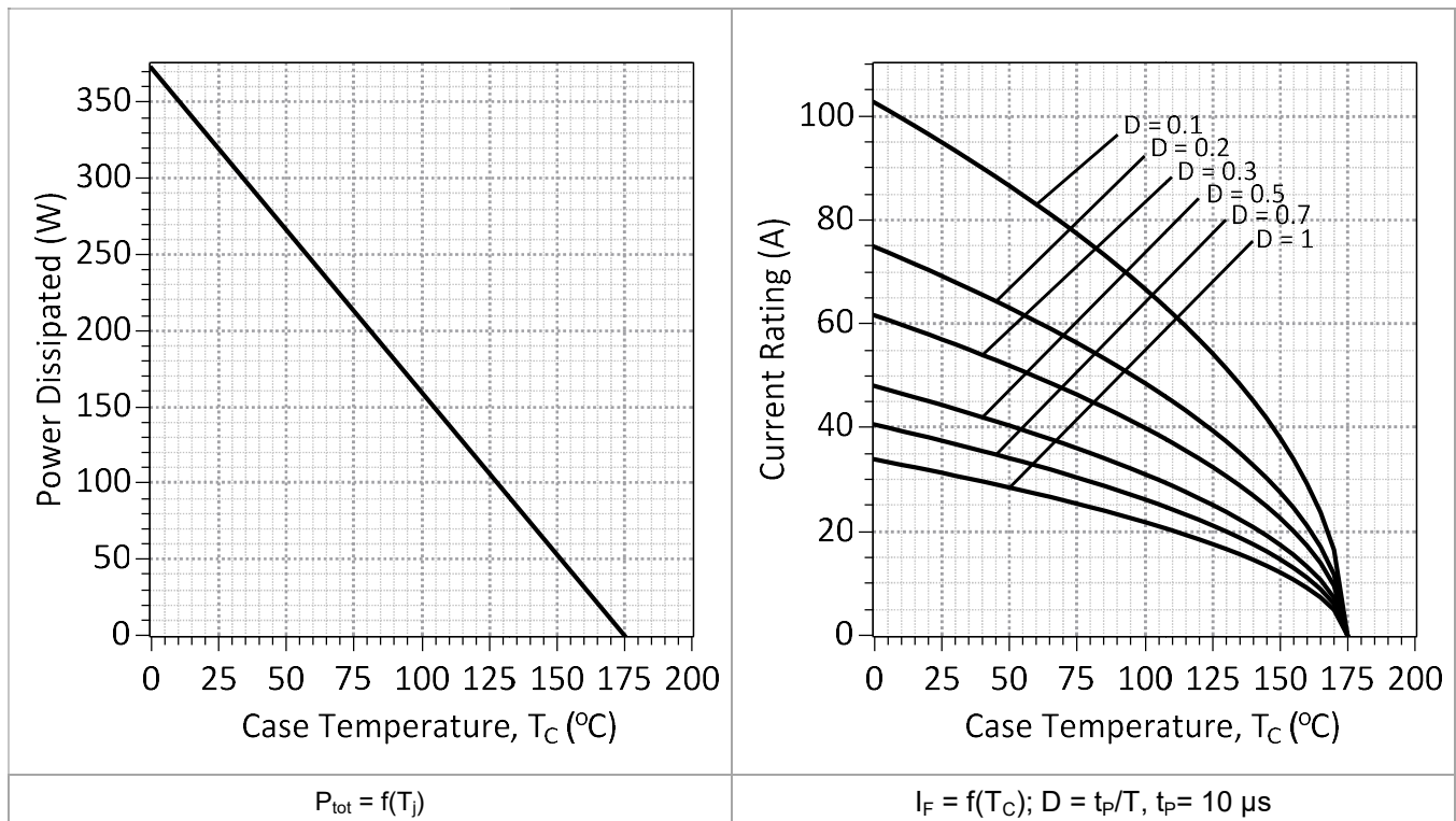
Figure 3: Power Derating Curve
