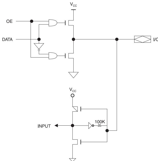
Figure 14. I/O diagram
