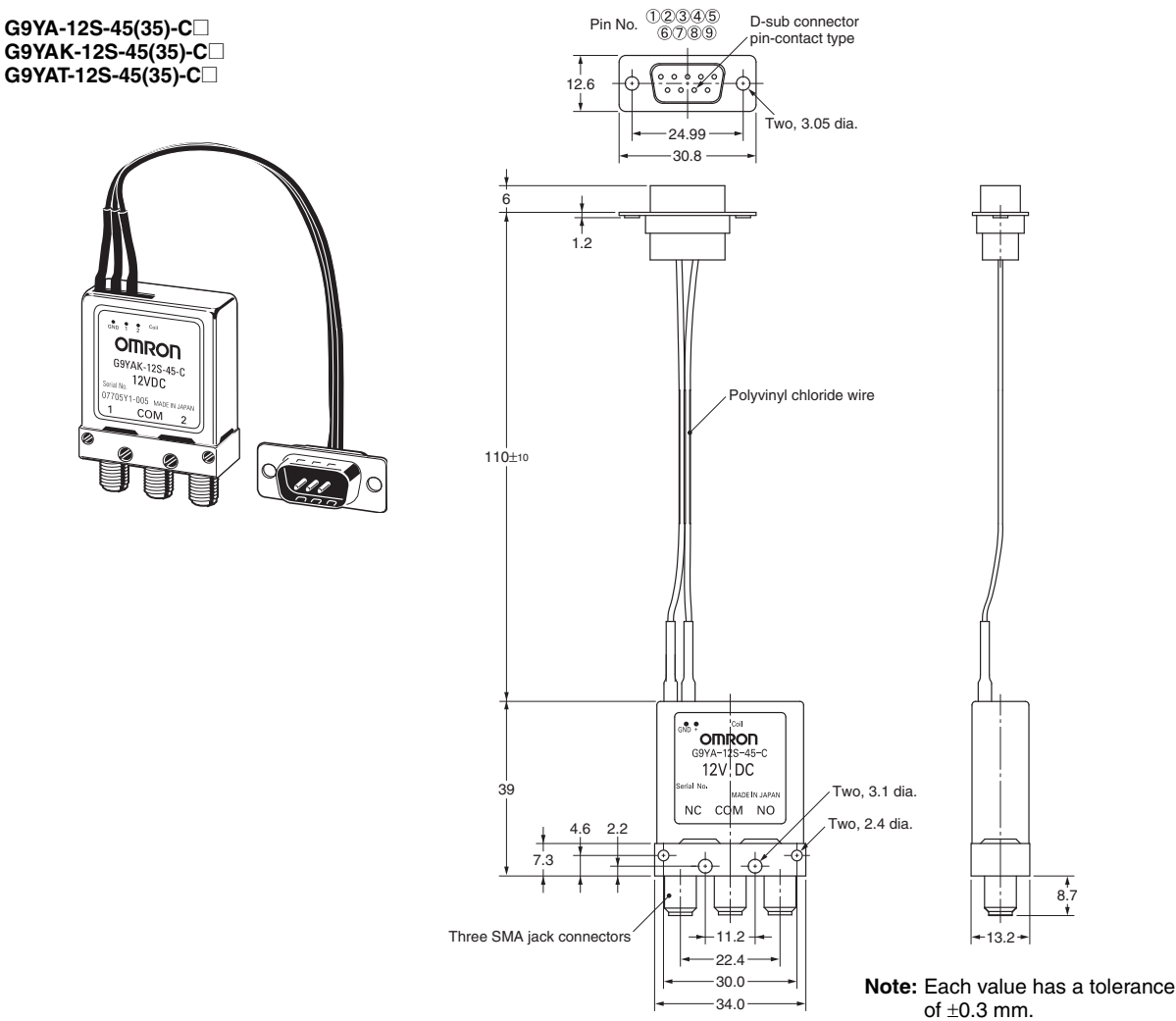
Pin Terminal Arrangement
