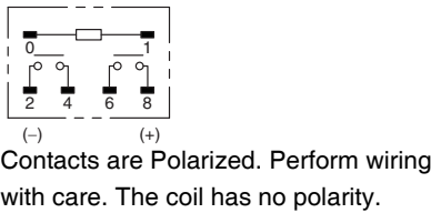
Two-pole Series Wiring Diagram (BOTTOM VIEW)
