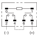
Two-pole Series Wiring Diagram (BOTTOM VIEW)
