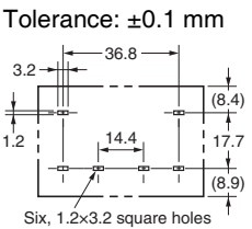
PCB Mounting Holes (BOTTOM VIEW)
