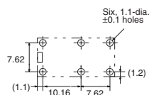
Mounting Holes (Bottom View)
