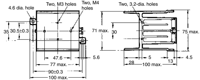
Mounting Holes
