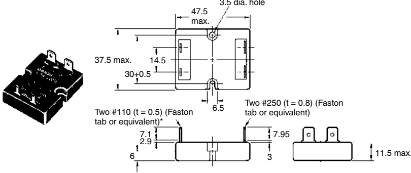
G3NE-205T(L)/210T(L)/220T(L)-(-2)(US)
