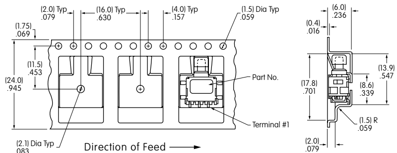
Tape Dimensions
