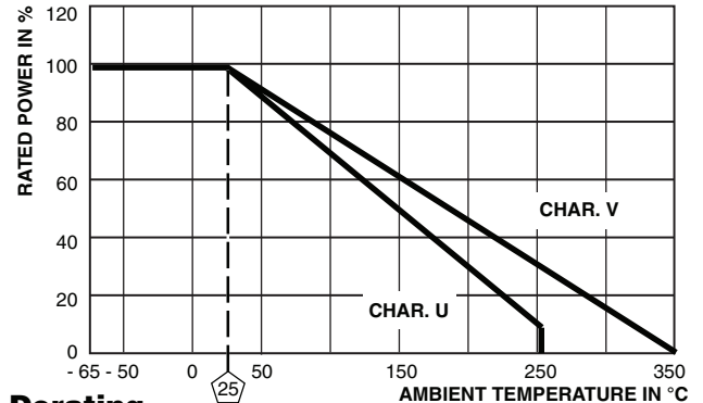
Derating
