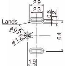
◆Recommended Board Termination Pattern
