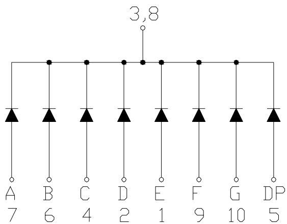
Common Cathode
