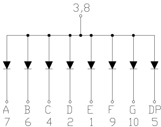
Common Anode
