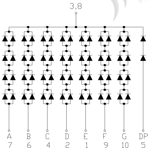
Common Cathode
