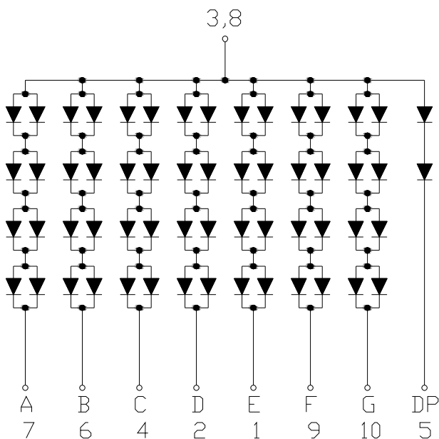
Common Anode
