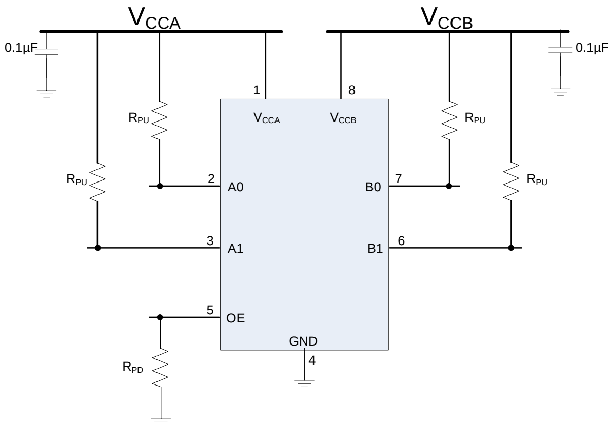
Figure 4. Application Circuit
