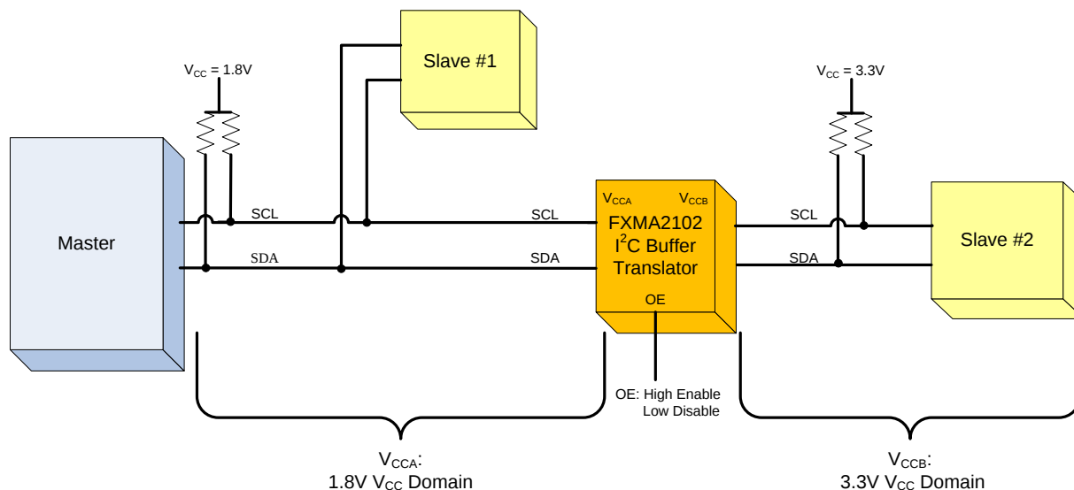
Figure 7. Bus Isolation
