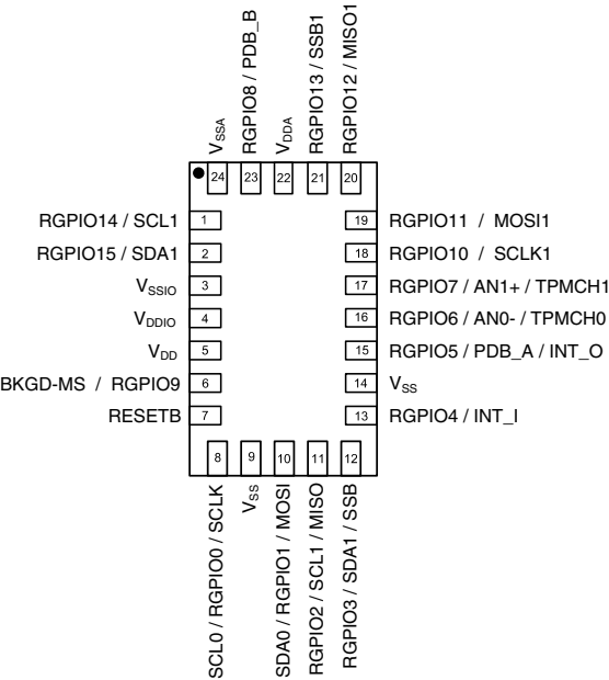
Figure 2. Device pinout (top view)
