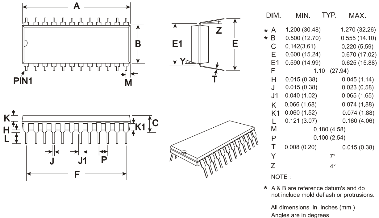
Figure 7 Mechanical Outline: Order as part no. FX828P4
