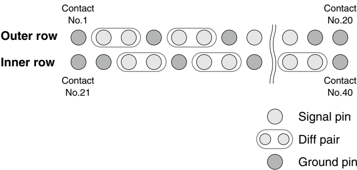
Pin assignment ( In case of 40 pos. )
