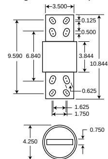
Fig. 3: 1200 Amp Range
