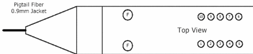
Figure 4 2×5SFF Planform
