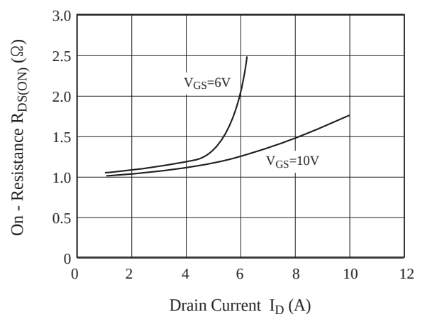
Fig4. R_{DS(ON)} - I_D
