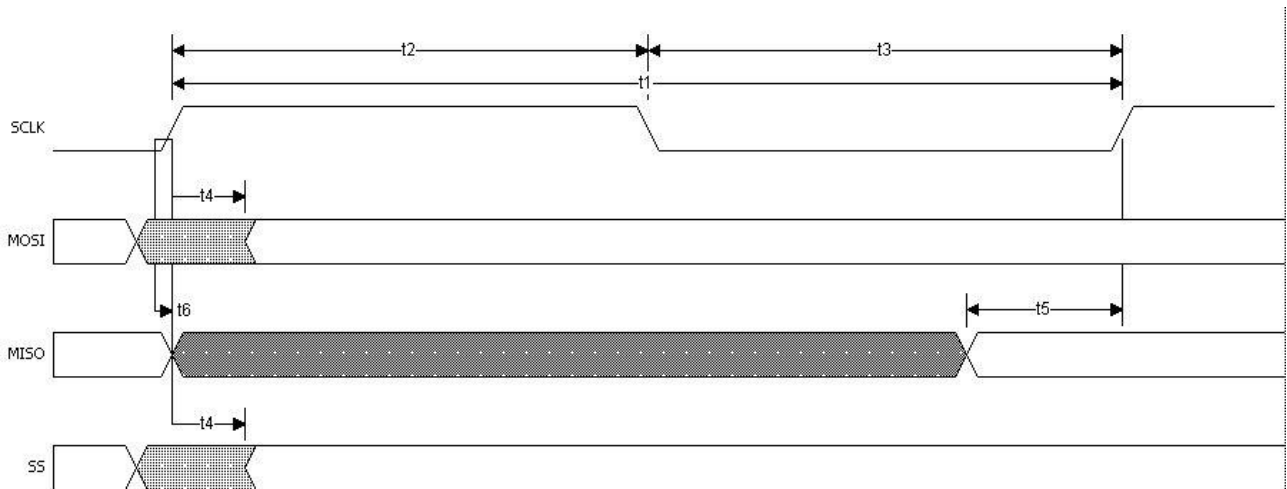
Figure 5-9 Typical SPI Master Timing
