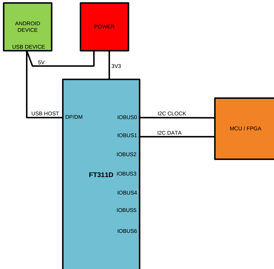
Figure 3.15 I 2 C Demo Block Diagram
