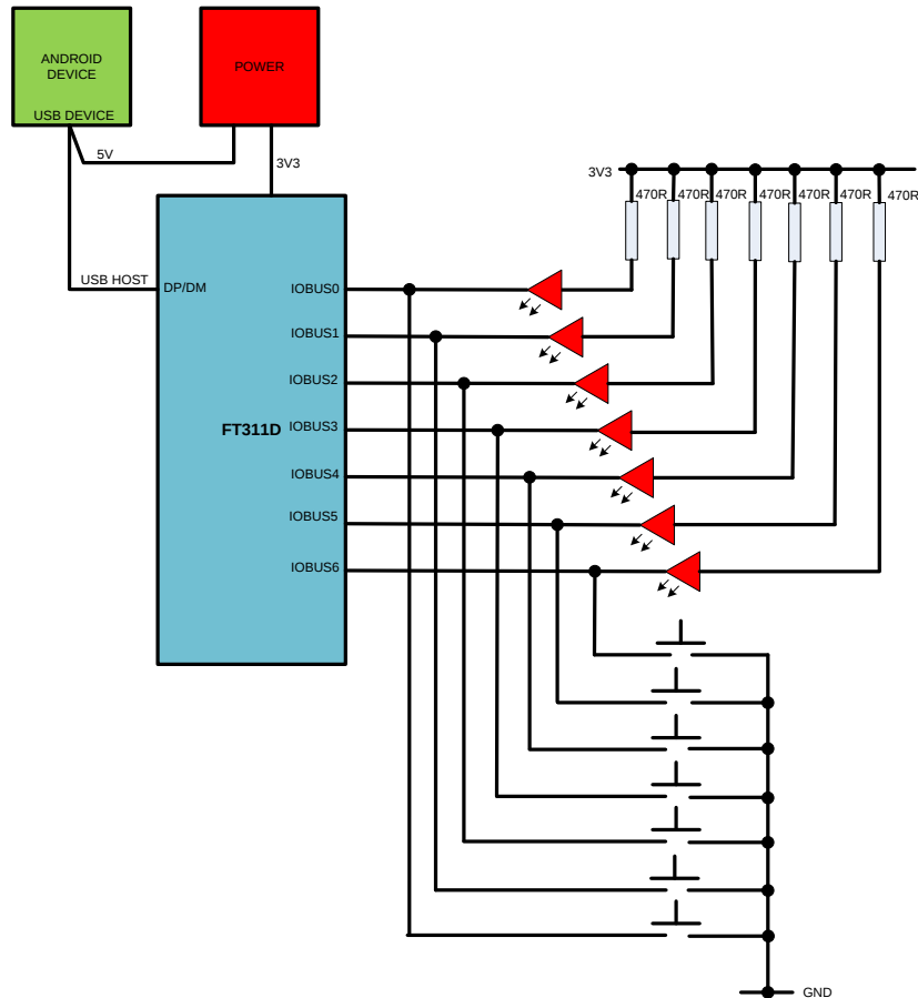
Figure 3.11 GPIO Demo Block Diagram
