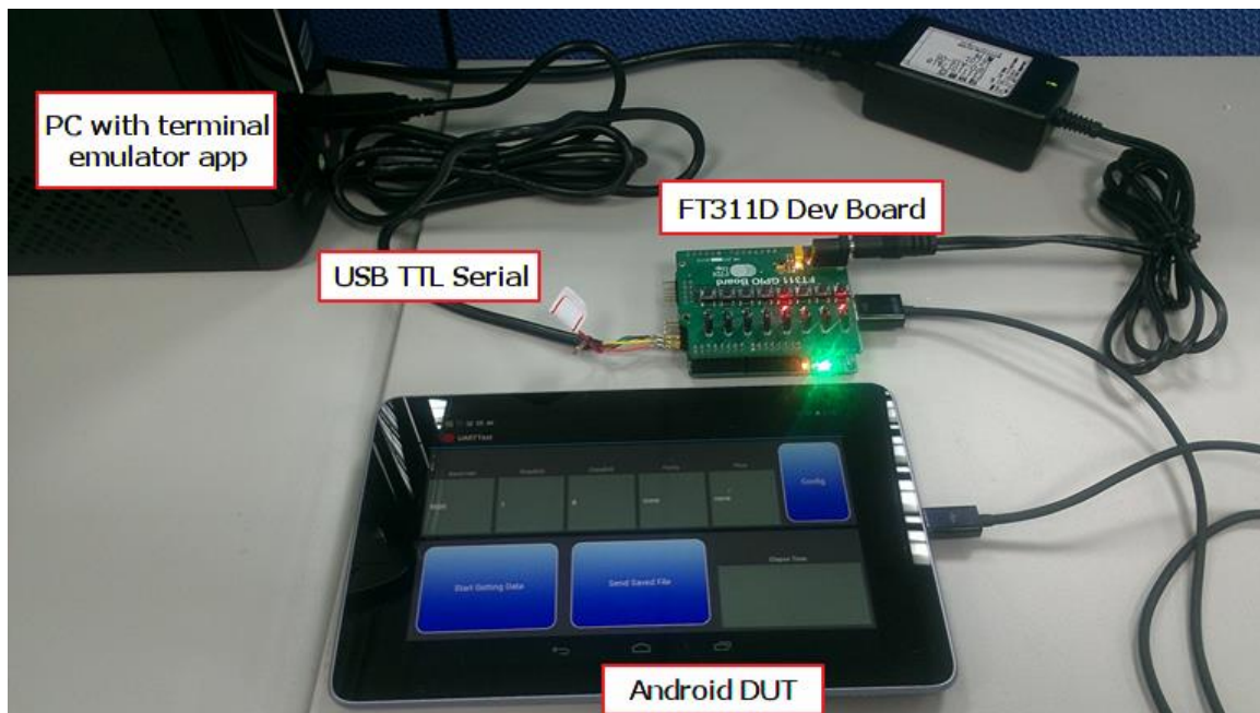
Figure 3.9 UART Test Setup
