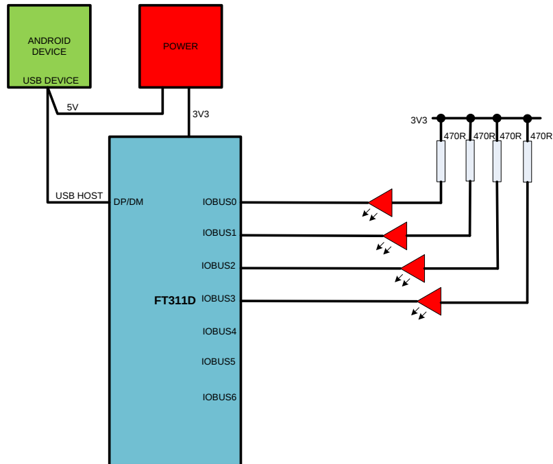
Figure 3.13 PWM Demo Block Diagram
