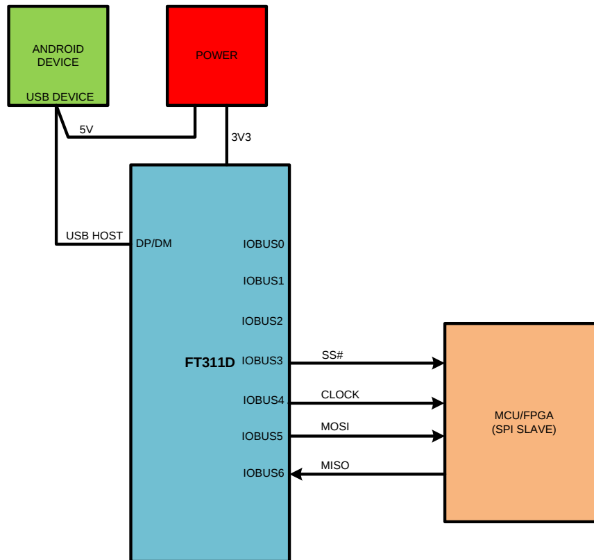
Figure 3.19 SPI Master Demo Block Diagram
