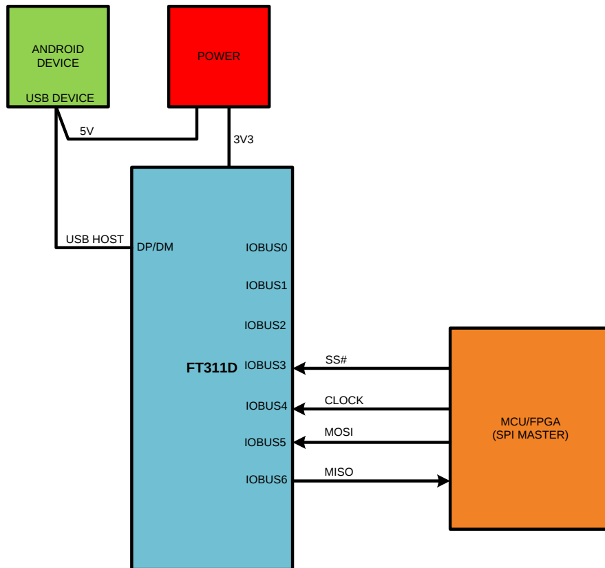
Figure 3.17 SPI Slave Demo Block Diagram
