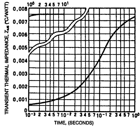
TRANSIENT THERMAL IMPEDANCE CHARACTERISTICS (JUNCTION TO SINK)
