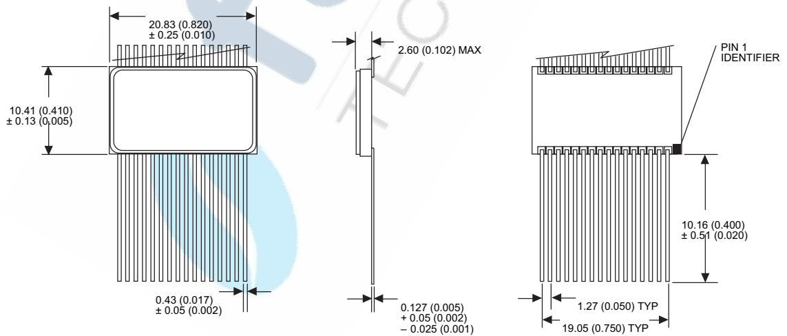
32 lead FP
