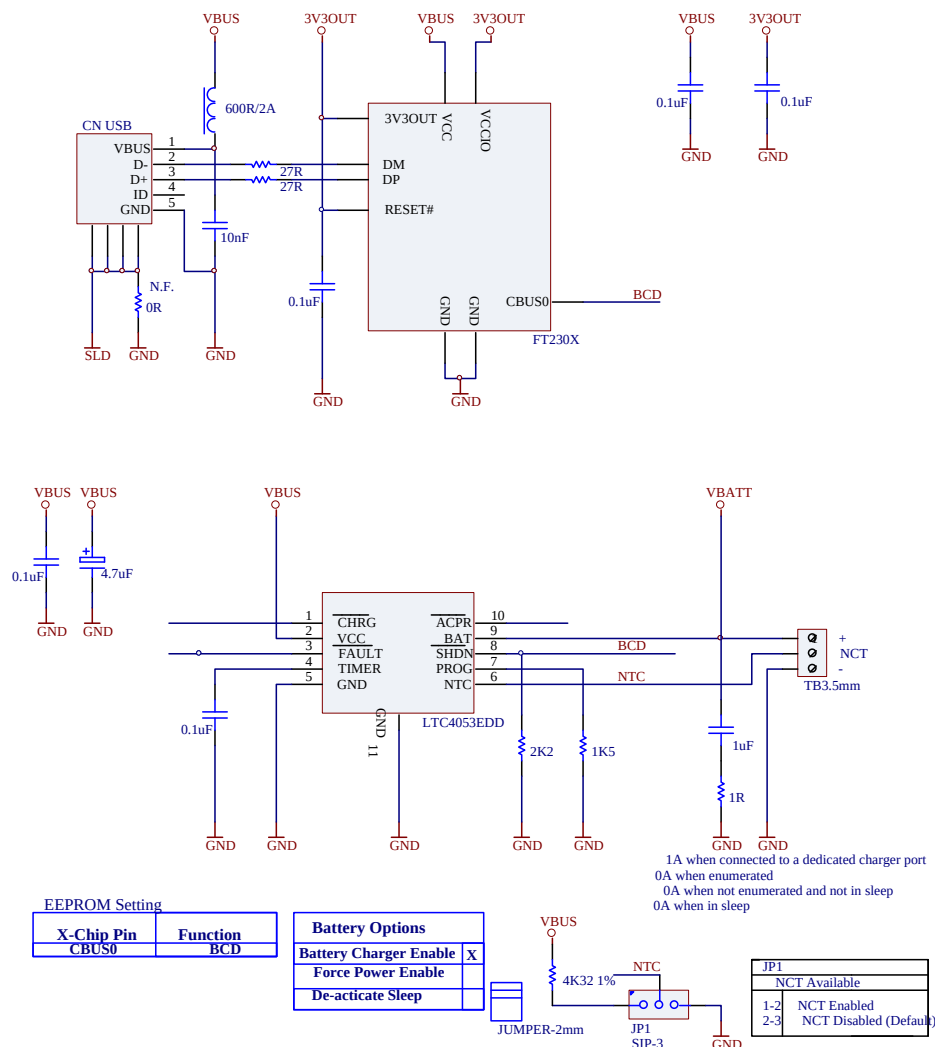
Figure 7.4 USB Battery Charging Detection (1 pin)
