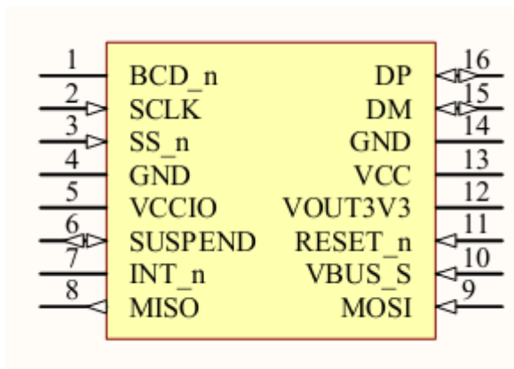
Figure 3-1 TSSOP-16 package schematic symbol
