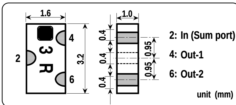
Shape & Size
