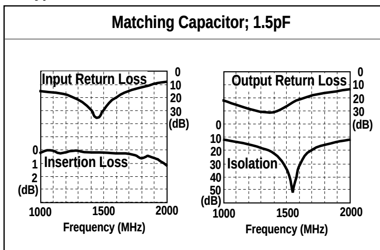
Typical Data
