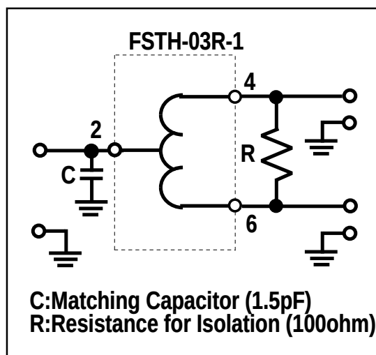
Measurement Circuit
