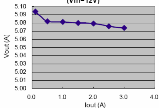
FSP3131 Load Regulation (Vin=12V)
