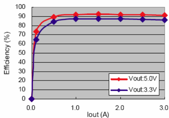
FSP3131 Efficiency
