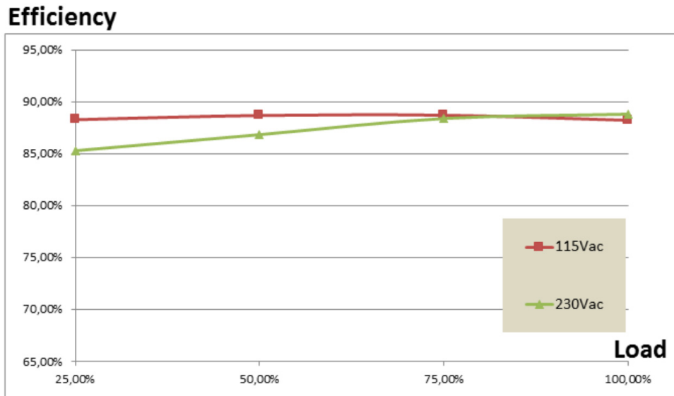
Figure 30. Board Efficiency
