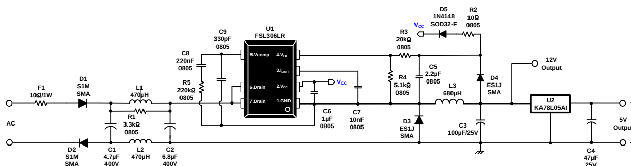
Figure 31. Schematic
