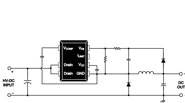
Figure 1. Buck Converter Application
