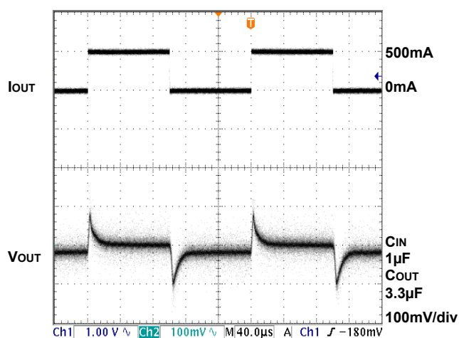
LOAD TRANSIENT
