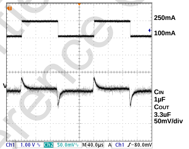
LOAD TRANSIENT
