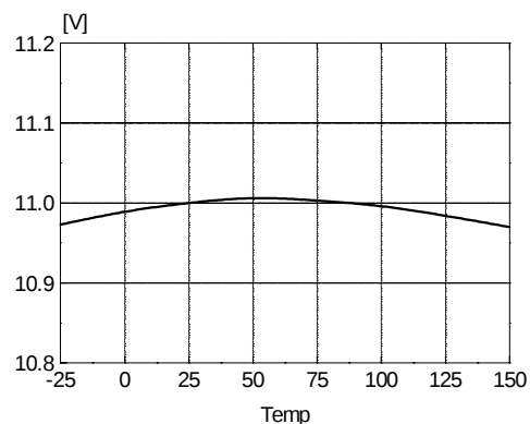
Figure 13. Burst Mode Low Voltage vs. Temp.
