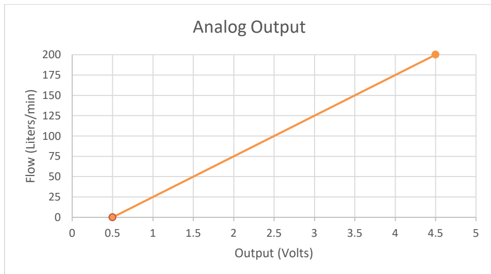
Figure 3. Analog Output
