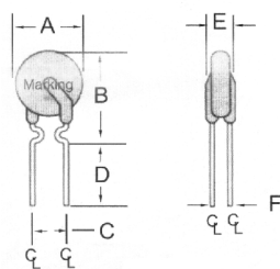
FRX010 ~ FRX090 Lead Size: 24AWG (0.5mm)
