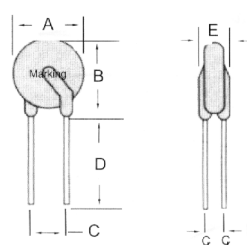
FRX110 ~ FRX375 Lead Size: 20AWG (0.81mm)
