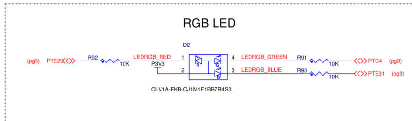
Figure 10. RGB schematic diagram
