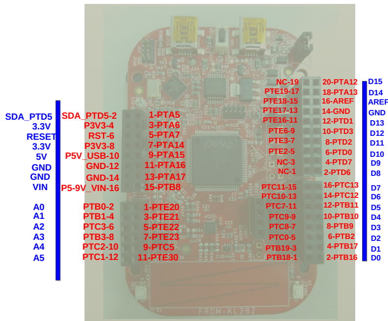
Figure 15. Input/output headers
