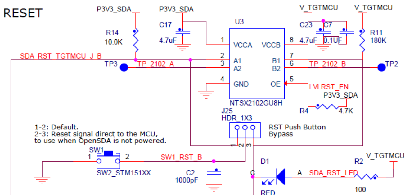
Figure 16. Reset circuit
