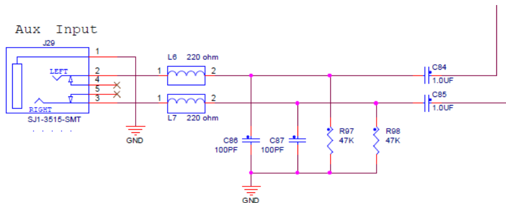
Figure 22. FRDM-K66F AUX_IN
