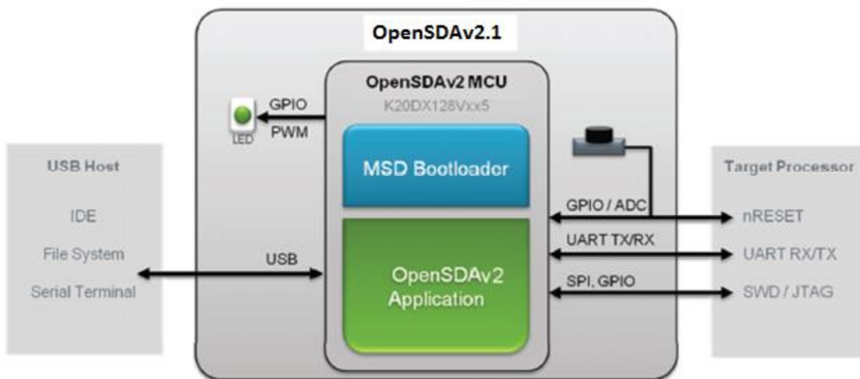
Figure 4. OpenSDA high-level block diagram
