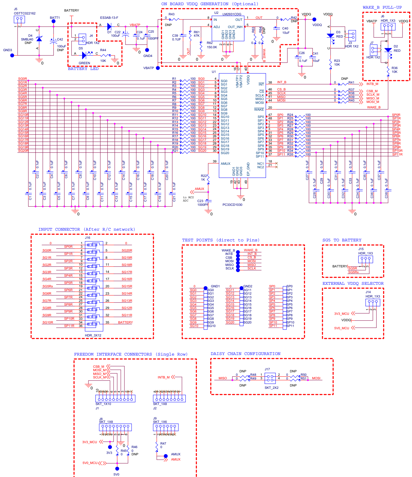
Figure 4. Schematic
