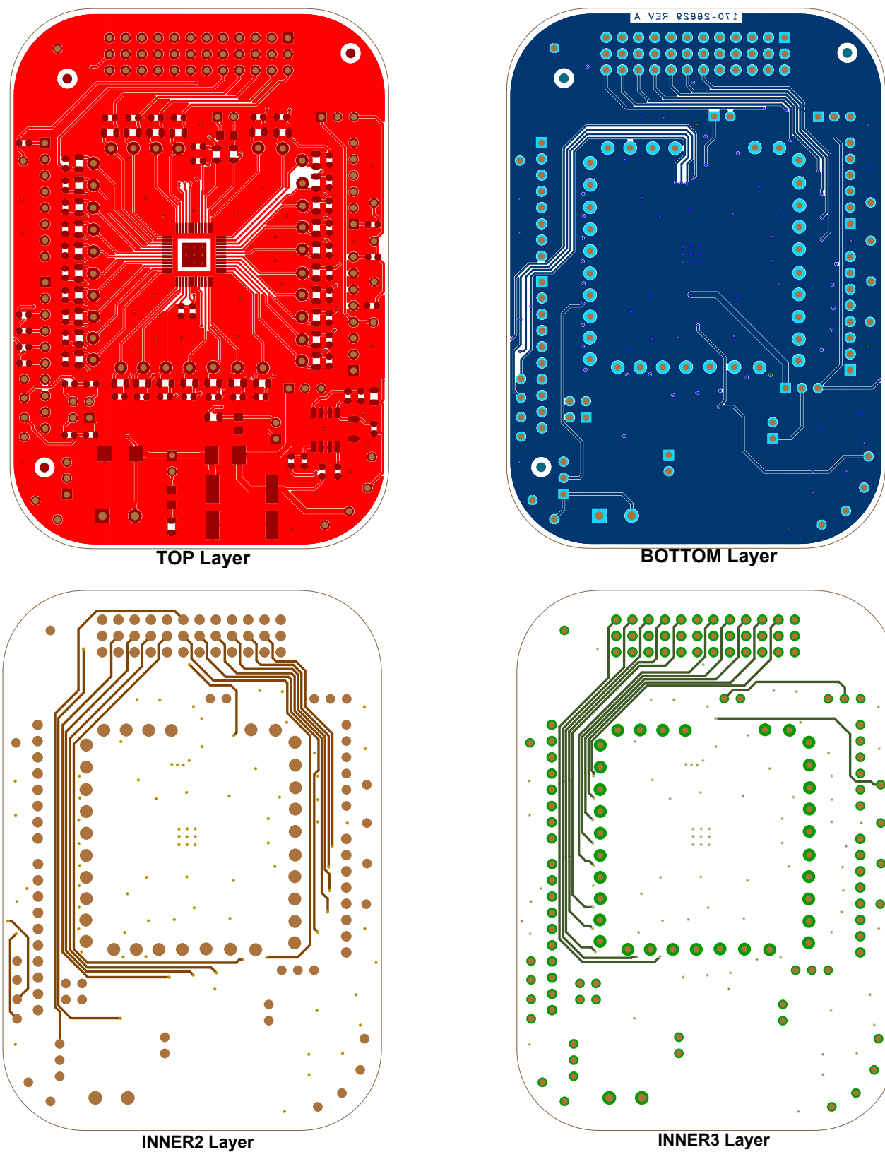
Figure 5. Layout
