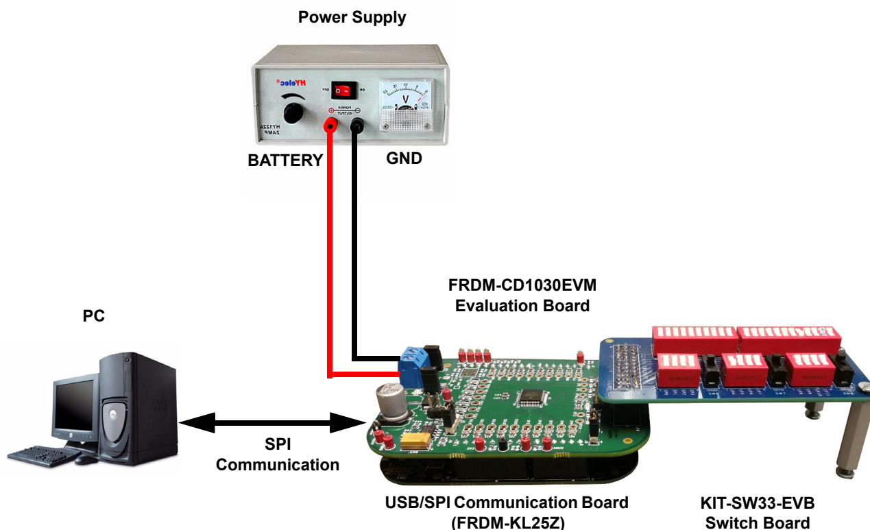
Figure 11. Evaluation Kit Setup
