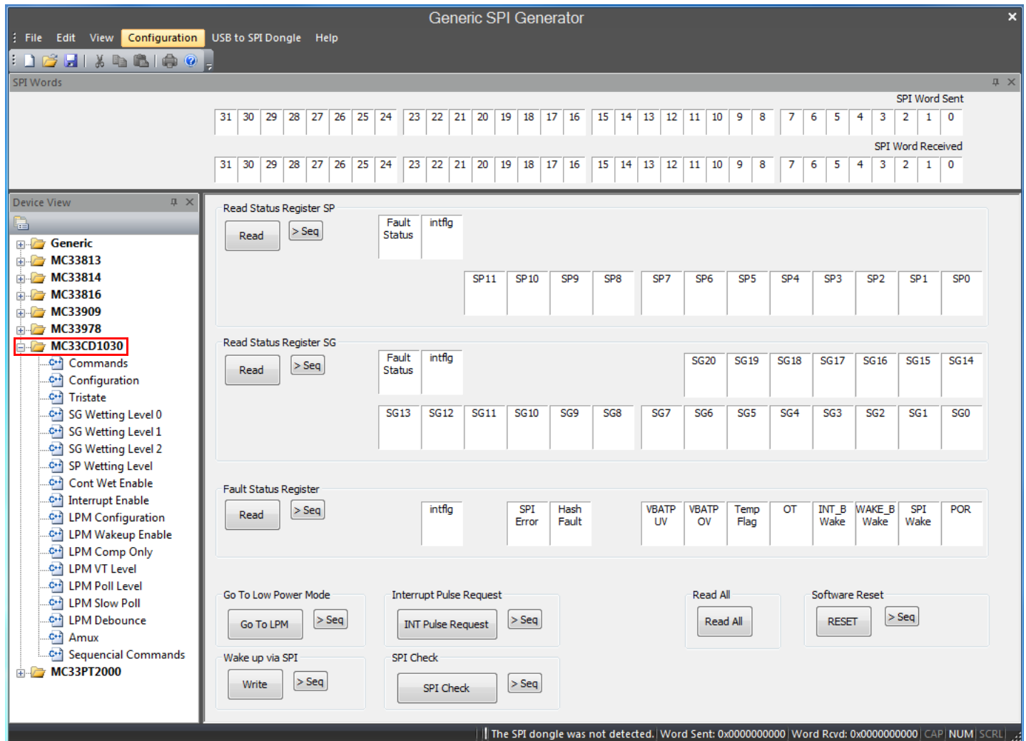
Figure 12. SPIGen GUI
