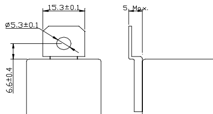
METAL BRACKET DUST COVER
