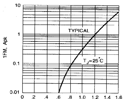
Fig. 3 - FORWARD CHARACTERISTICS
