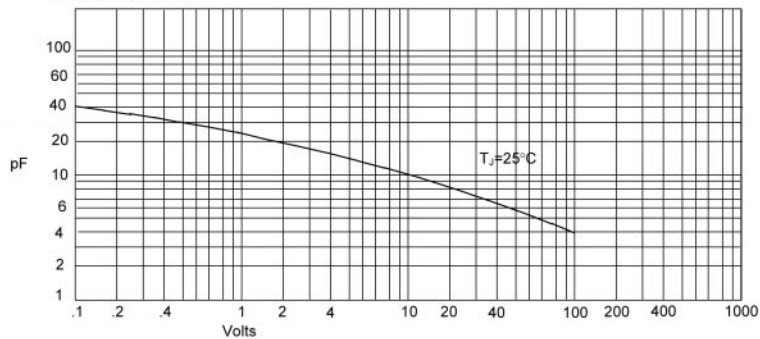
Figure 3 Junction Capacitance
