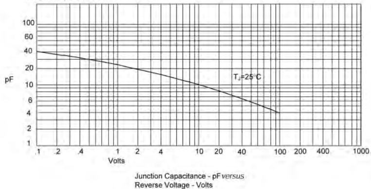
Figure 3 Junction Capacitance
