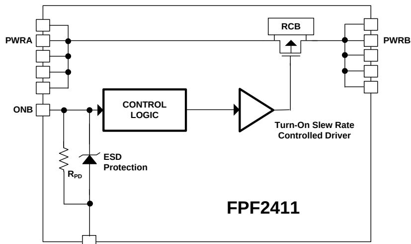
Figure 3. Block Diagram
