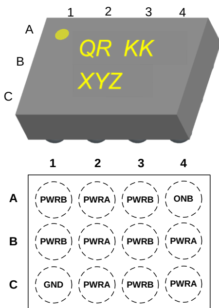
Figure 5. Top View
