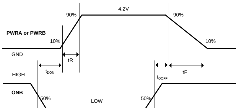
Figure 4. Dynamic Behavior
