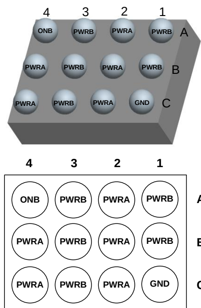
Figure 6. Bottom View
