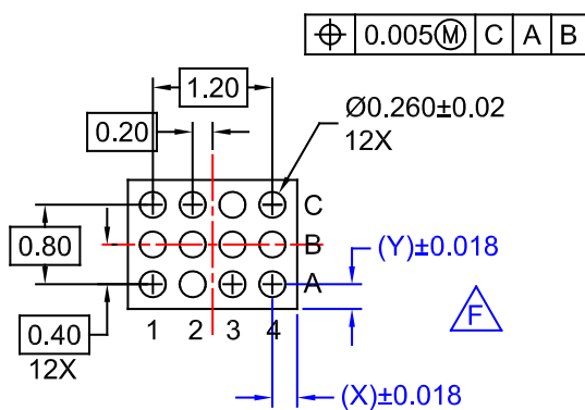
Figure 6. 12-Ball, 3×4 Array, 0.4 mm Pitch, Wafer-Level Chip-Scale Package (WLCSP)
