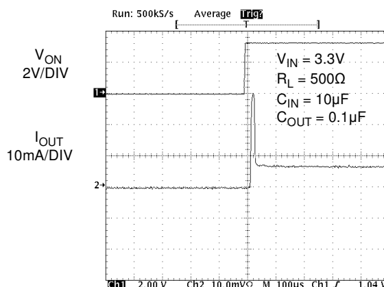
Figure 20. T_{ON} Response
