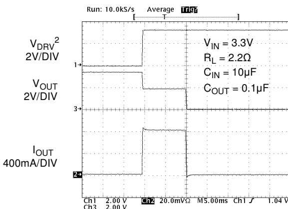
Figure 18. T_{BLANK} Response
