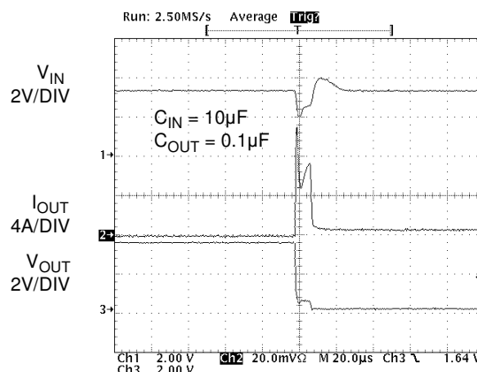
Figure 22. Short Circuit Response (Output Shorted to GND)
