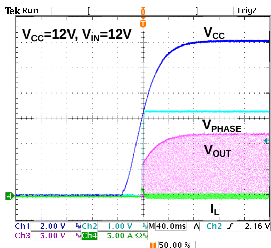
Figure 8. Power On at 0A Loading
