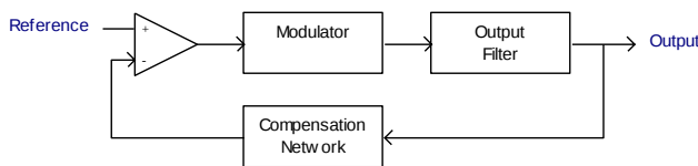
Figure24. Basic structure of the buck converter
