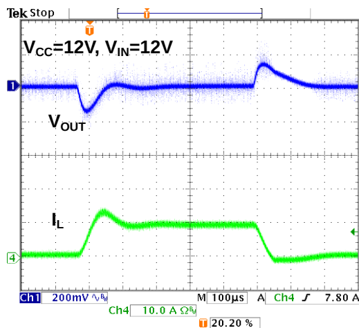
Figure 18. Transient test: Slew rate:2.5A/μs, (1A to 10A)
