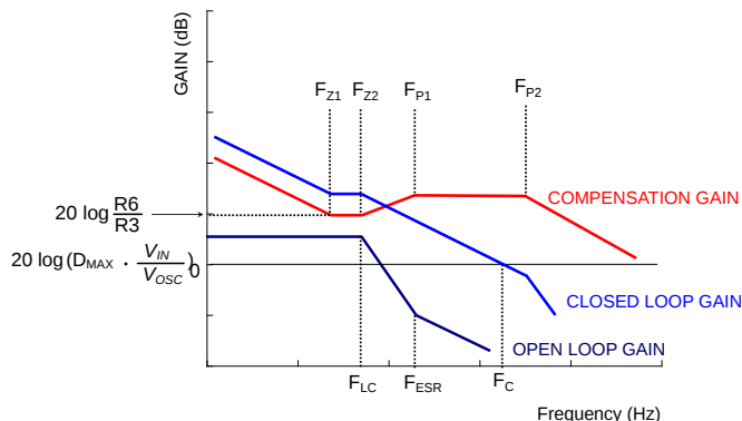
Figure 27. Bode plot of converter closed loop gain
