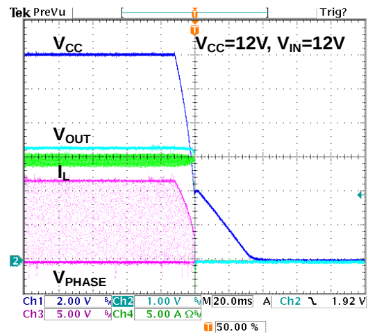
Figure 11. Power OFF at 15A Loading
