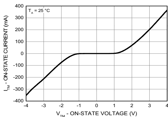
Fig 9. On-State Characteristics
